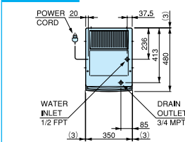
Air Flow : Bottom in / Top out
