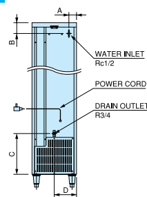
Air Flow : Front in / Back side out
